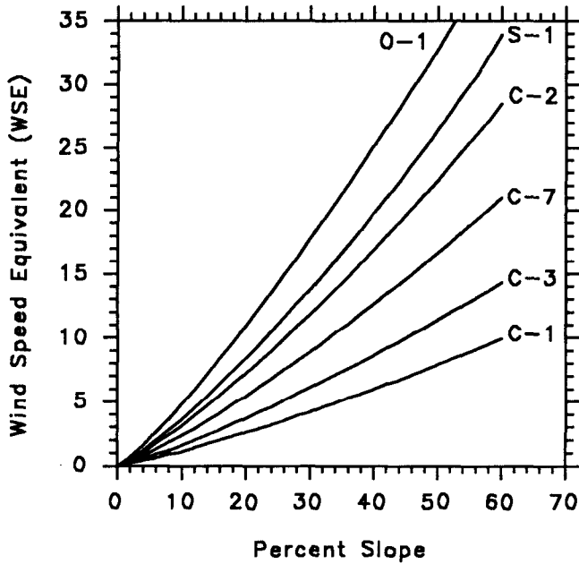
Figure 12. Equivalent wind speeds of measured percent slope for several fuel types; FFMC has been set to 89.
